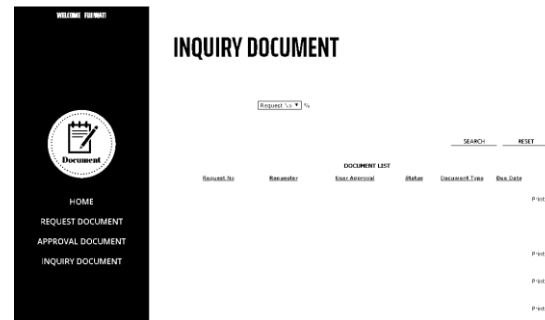
Gambar 6. Halaman document
