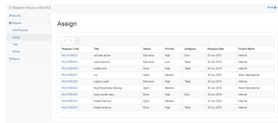
Gambar 8. Tampilan assign
