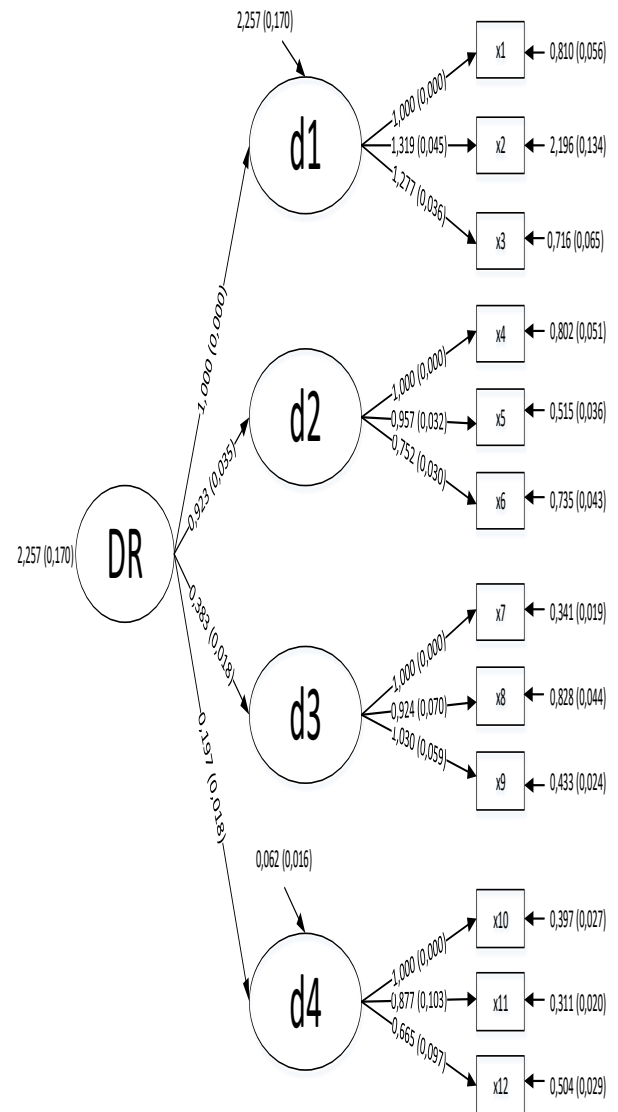
Gambar 3. CFA model pengukuran variabel DR.
