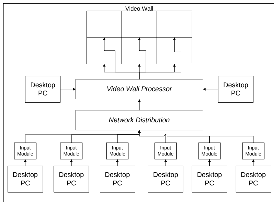
■ Gambar 4. Arsitektur Hybrid Video Wall Processing.
