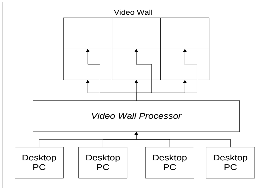
■ Gambar 1. Arsitektur Centralized Video Wall Processing.
