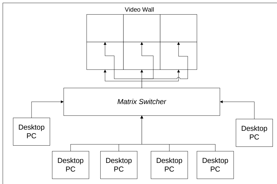
■ Gambar 2. Arsitektur Matrix Switcher Distribution.
