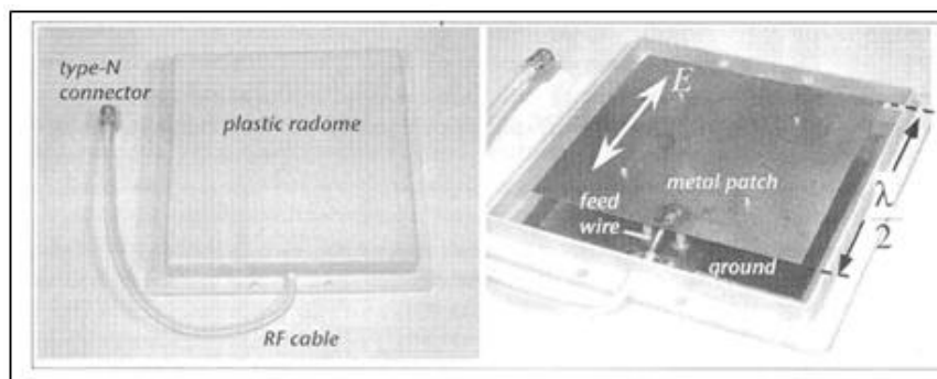
■ Gambar 9. Antena tipe patch RFID reader
