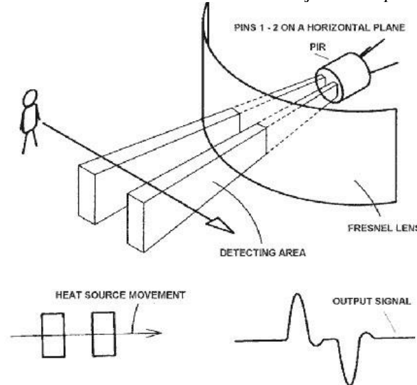
■ Gambar 7. Cara Kerja Sensor passive infrared receiver (PIR)
