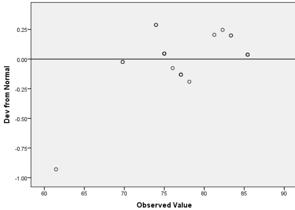
Detrended Normal Q-Q Plot of Nilai for Kelas= Kelas Kontrol
