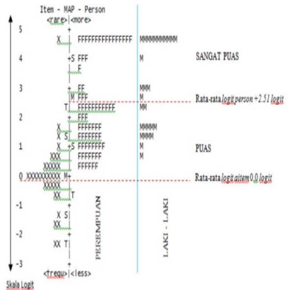
Fig 6. Wright Map with Rasch model according to satisfication service of female and male
