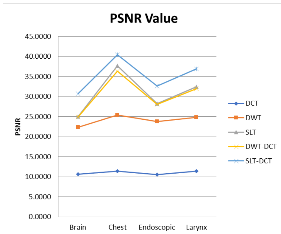
Figure 9. PSNR Value of Tested Images
