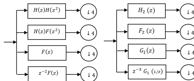
Figure 2. Comparison of Two-Scale Iterated D_2 Filterbank (left) and Two-Scale Filterbank (Right) [3]
