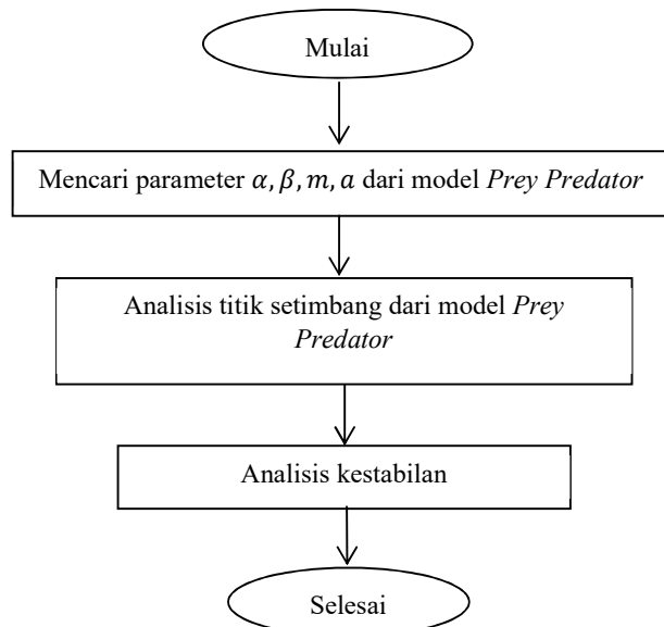
Gambar 1. Flowchart penelitian
