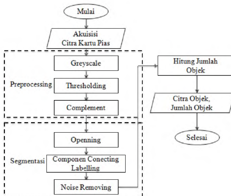
Gambar 4. 1. Flowchat system
