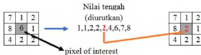
Gambar 3. 3. Median filter
