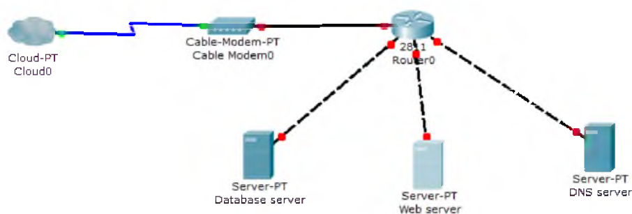
Gambar 2 Deployment Diagram Sistem Pengujian VLSM
