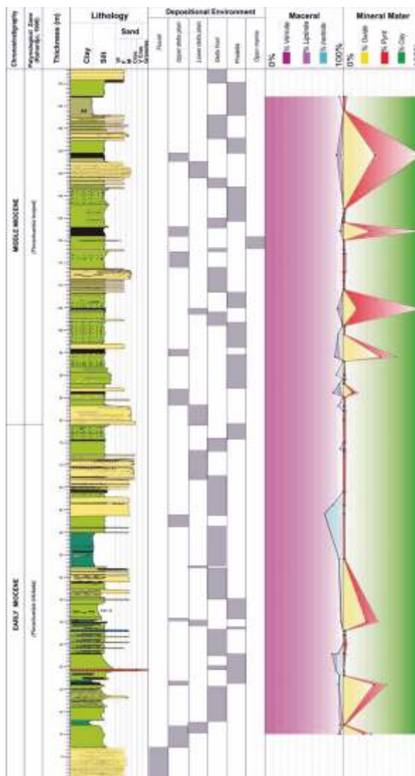
Figure 9. Vertical variations of maceral and mineral matter compositions within the organic rich sediments of the Balikpapan Formation in the Palaran section.
