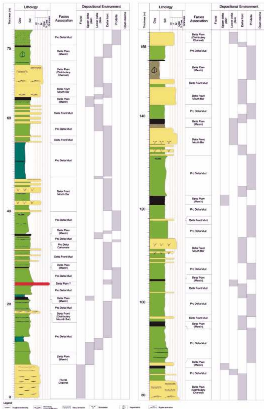
Figure 3. Stratigraphic measured section of the Palaran area, showing lithological variation, contains of shale-coal and sandstones cycles, represent complete cycles of fluviodeltaic depositional environment in the studied area.
