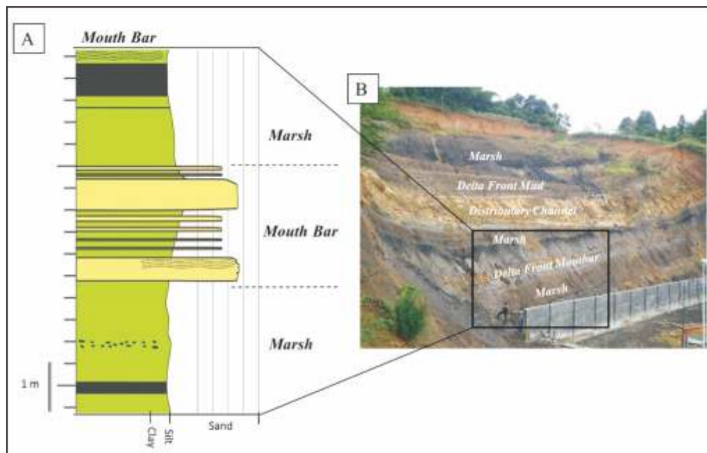
Figure 4. Outcrop expressions of cyclic facies association in the lower part of the Loa Janan section; A) stratigraphic log showing upper delta plain marsh and delta front mouth bar facies association; delta plain marsh comprise of thick facies interbedded by thin coal bed seam, while the delta front mouth bar composed of fine to medium grained sandstones, with coarsening and thickening upward trends; B) outcrop photograph represent deltaic cycle environment, facies changes from the fluvial dominated upper delta plain marsh, to tidal influence lower delta plain and delta front.
