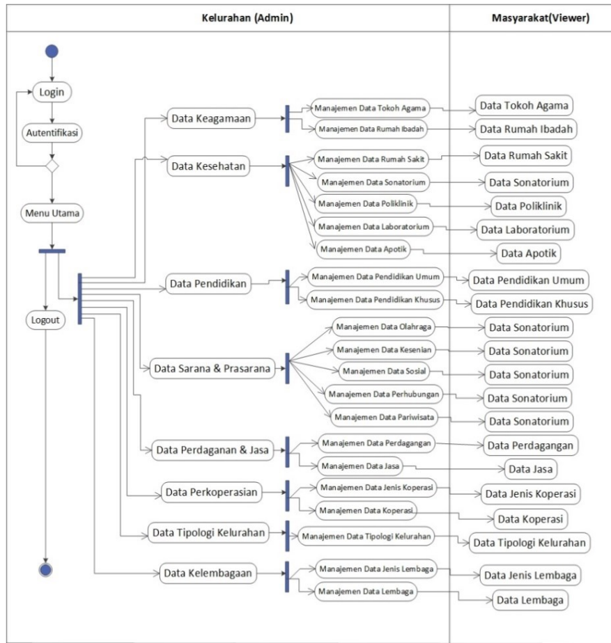
Gambar 3. Activity Diagram
