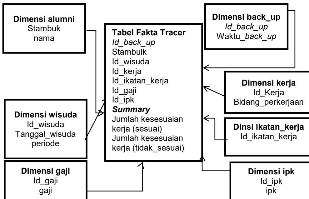
Gambar 2. Star skema Data Warehouse
