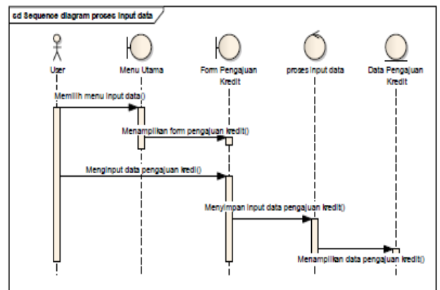
Gambar 6. Sequence Diagram Proses Input Data
