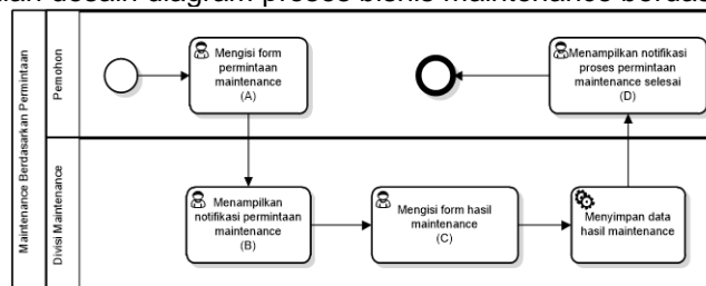
Gambar 11. Diagram proses bisnis Maintenance Berdasarka Permintaan
