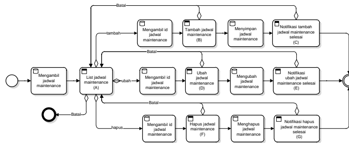
Gambar 3. Sub Diagram proses bisnis Jadwal Maintenance
