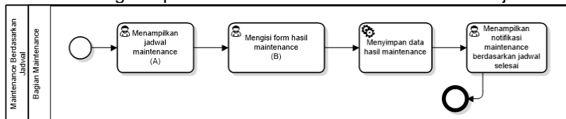
Gambar 14. Diagram proses bisnis Maintenance Berdasarkan Jadwal
