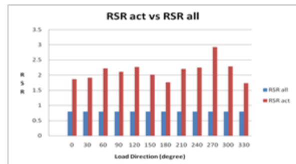
Figure 7. Comparison between predicted (actual) RSR and the allowable RSR
