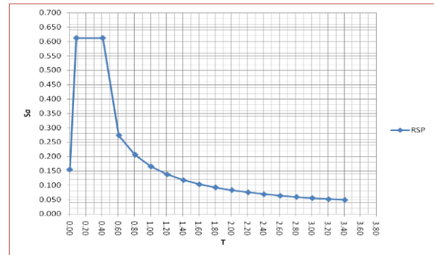
Figure 6. Response spectrum
