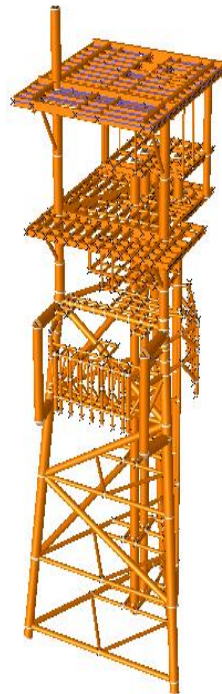
Figure 2. Results of structure modeling of overall ULA jacket platform
