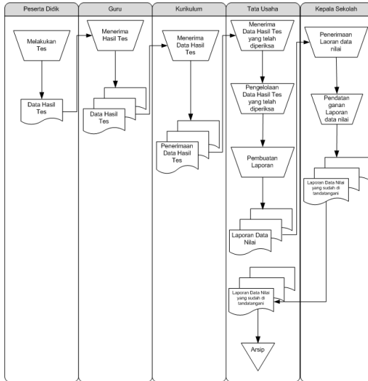
Gambar 3. Flowmap Penilaian
