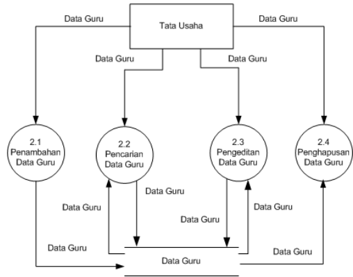
Gambar 4.4 DFD Level 1 Proses 2 Pengolahan Data Guru
