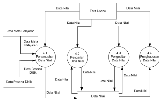
Gambar 4.6 Data Flow Diagram (DFD) Level 1 Proses 4 Pengolahan Data Nilai
