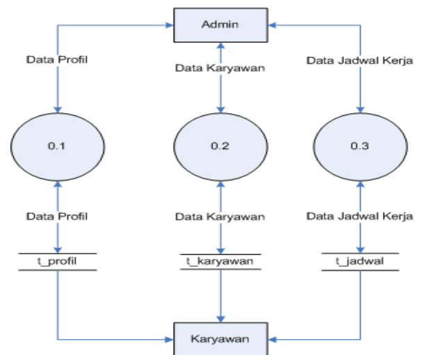
Gambar 5. Diagram Level 0
