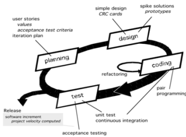
Gambar 2. Extreme testing Programming
