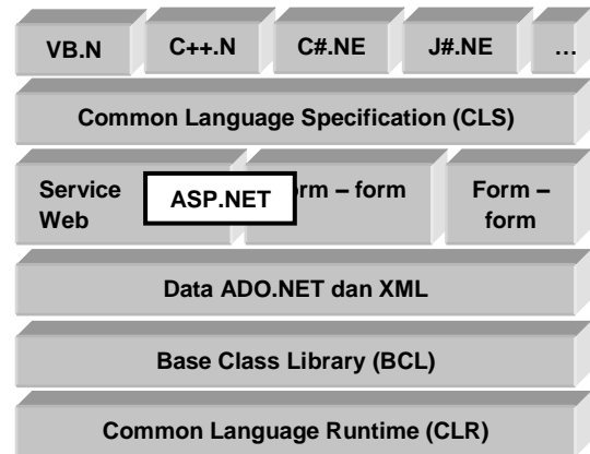
Gambar 2 Dot NET Framework
