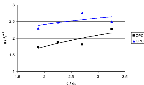
Figure 3. Comparison of the Bond Strengths of Geopolymer and OPC Concretes in Pull-out Tests
