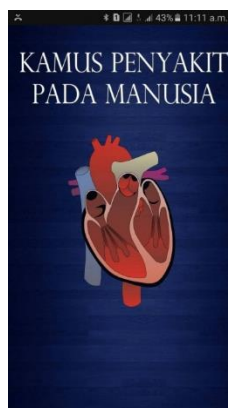
Gambar 14 Splash screen
