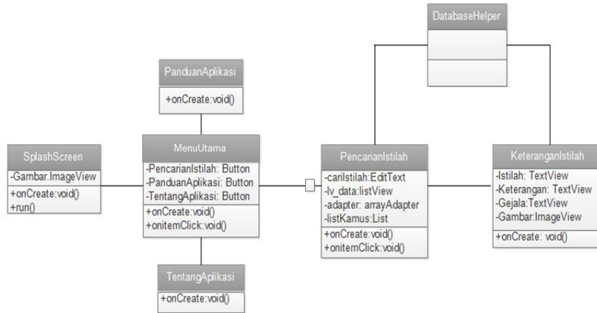
Gambar 5 Class diagram
