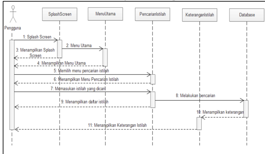
Gambar 7 Sequence diagram pencarian
