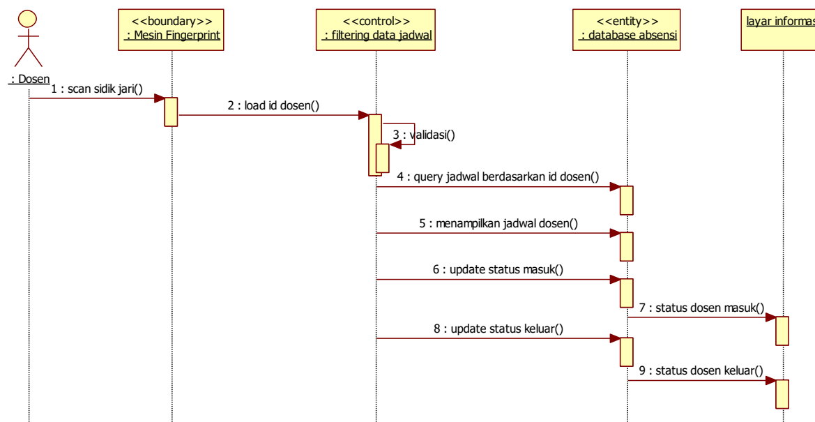
Gambar 7. Sequence Diagram Real time Absensi
