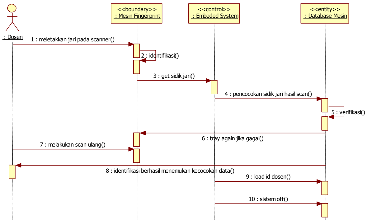
Gambar 6. Sequence Diagram Deteksi Sidik Jari
