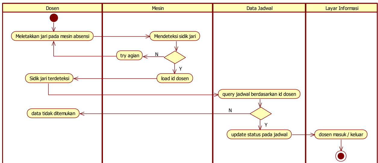
Gambar 5. Activity Diagram Real time Absensi
