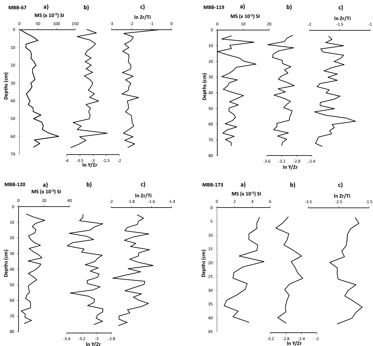
Figure 5. Vertical variations of magnetic susceptibility, \ln Y/Zr , \ln Zr/Ti of cores MBB-67 (top left), MBB-119 (top right), MBB-120 (bottom left) and MBB-173 (bottom right).
