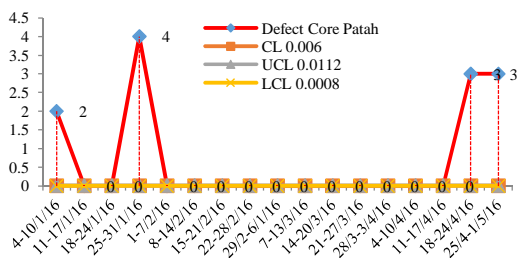
Gambar 5. Diagram Core Patah
