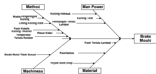
Gambar 12. FMEA Defect Brake Mould
