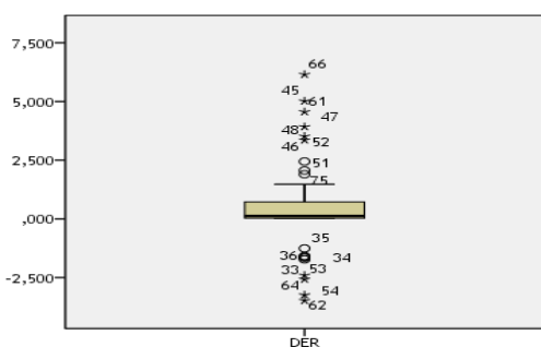
Gambar 1. Boxplots-DER
