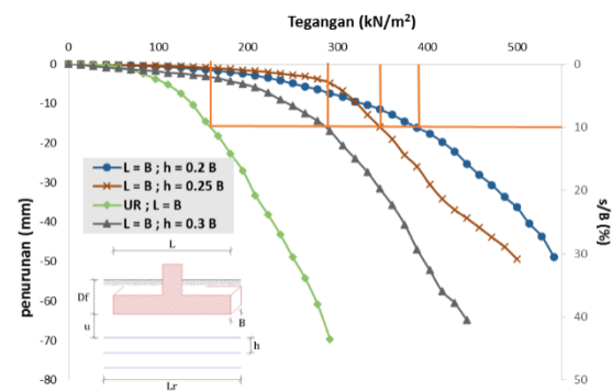
(a) L/B = 1
