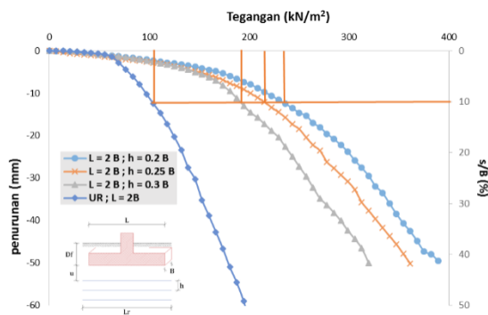
(c) L/B = 2
