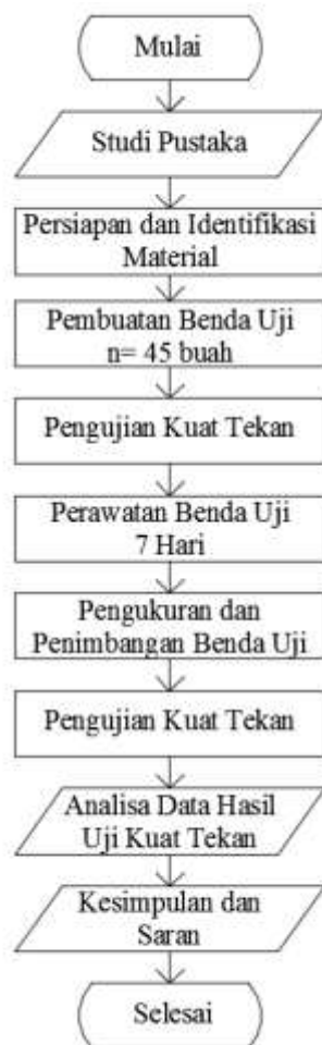
Gambar 5. Diagram alir penelitian beton porous.
