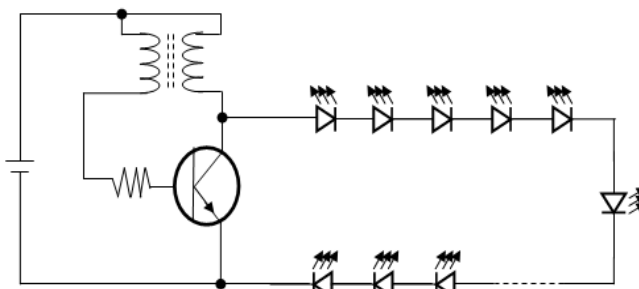
Figure 4. Serial LEDs Load Circuit
