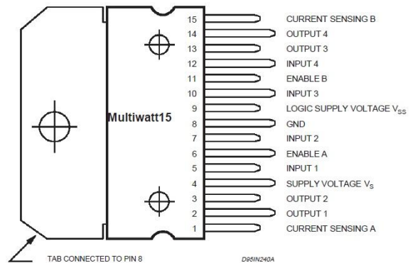
Fig. 3. L298N pin structure.
