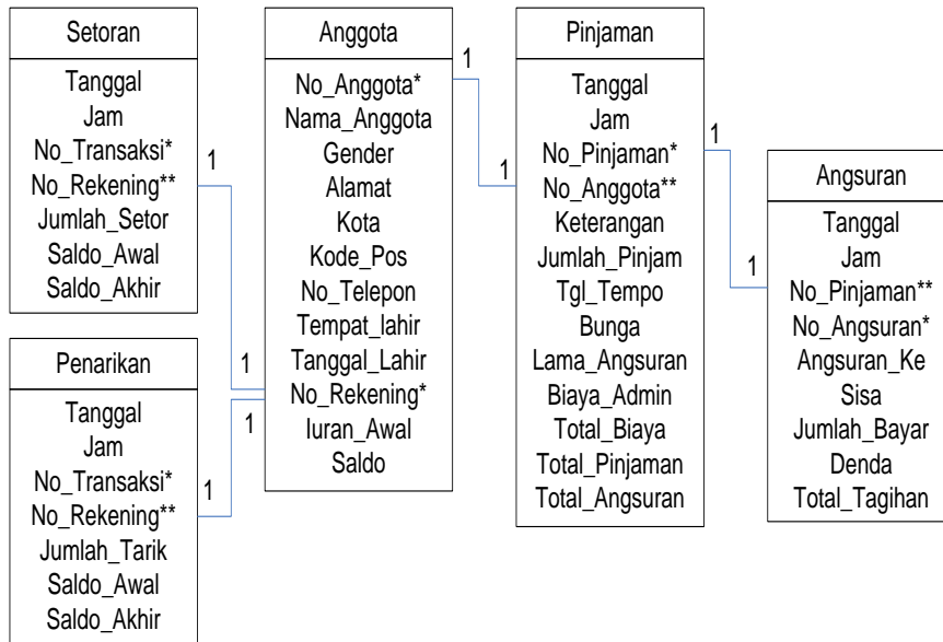
Gambar 3. Logical Record Structure (LRS)
