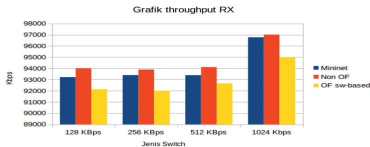
Gambar 10. Grafik TCP Throughput Rx
