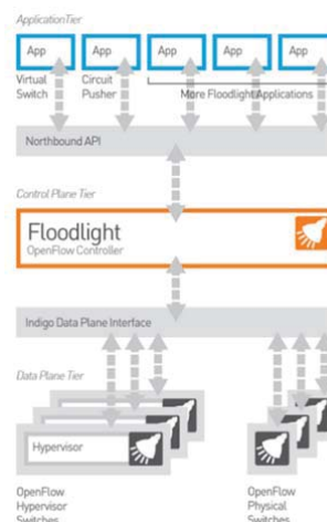
Gambar 4. Floodlight framework (Sumber: http://www.projectfloodlight.org/floodlight/ )
