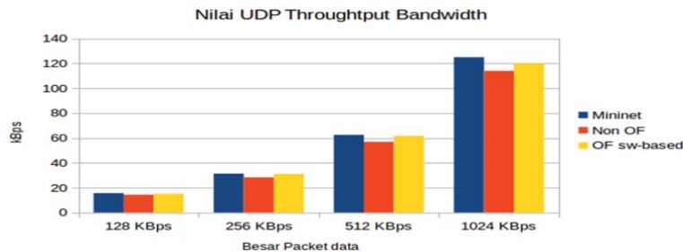
Gambar 11. Grafik Nilai UDP Throughput bandwidth
