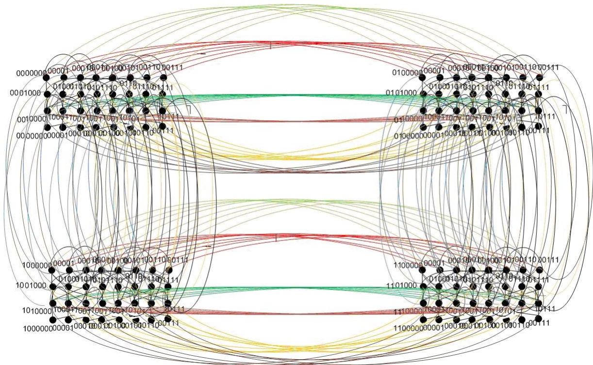
Gambar 1: Torus Butterfly (2,2,3)[3]
