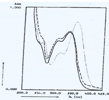
Gambar 4 Spektra flavonoid A1 dalam MeOH, NaOAc dan H 3 BO 3 --- = MeOH : 250, 300 s , 325 .... = MeOH+NaOAc : 253, 300 s , 325 ..... = MeOH+NaOAc+ H 3 BO 3 :256,303 s ,350
