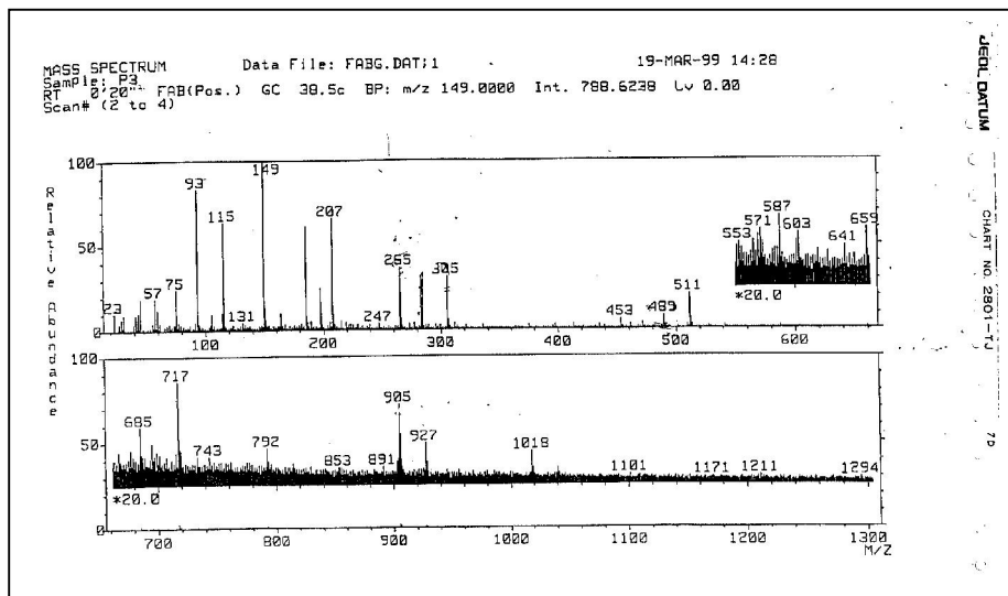
Gambar 10. Spektrum massa Flavonoid A1
