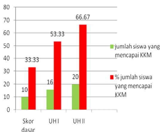
Gambar 4.1: Diagram Analisis Ketercapaian KKM
