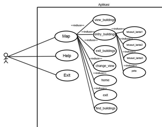
Gambar 3. Use Case Diagram Aplikasi Peta 3D UNIMA
