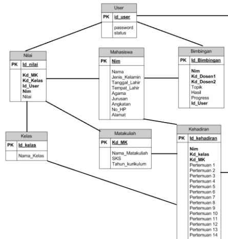
Gambar 8. Konseptual Database
