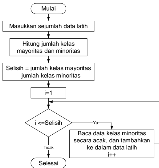
Gambar 3 Flowchart Algoritma ROS (Random Oversampling)
