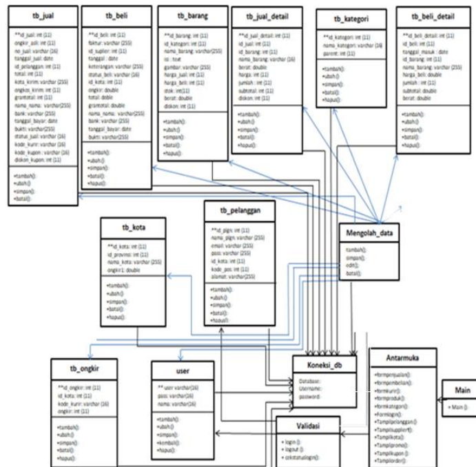
Gambar 3. Class Diagram Sistem
