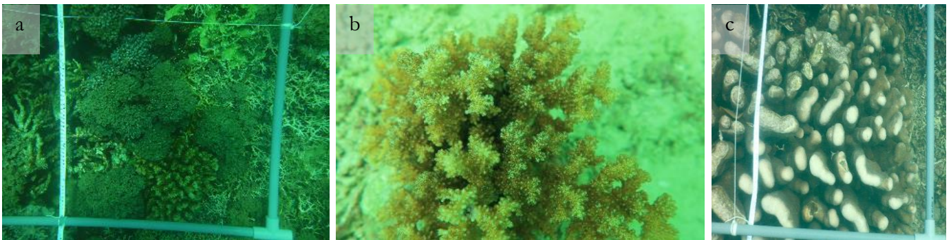
Figure 8. Family Pocilloporidae (a, b) and Psammocoridae (c).
