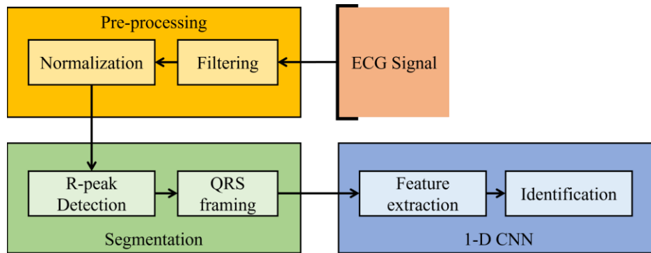
Fig. 2. The block diagram of the proposed model
