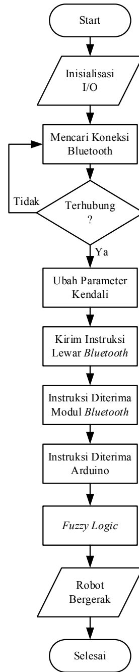
Gambar 8. Flowchart sistem
