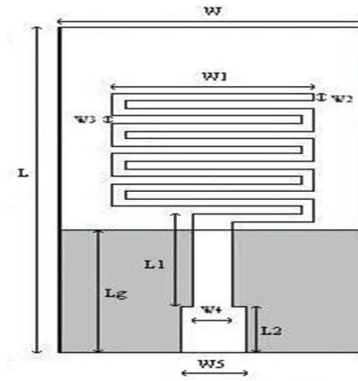
Gambar 1. Mikrostrip Meander-line
