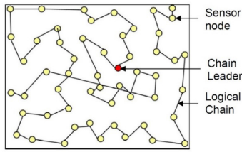
Gambar 3. PEGASIS network model
