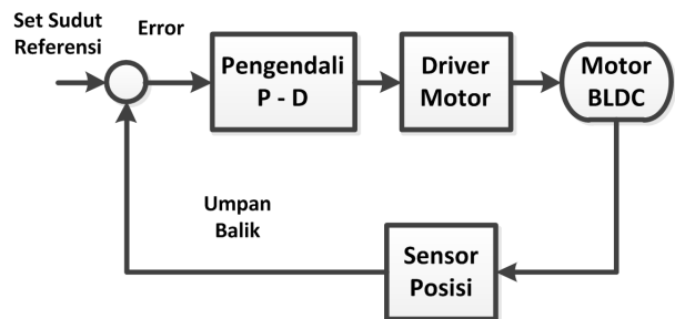
Gambar 3. Diagram pengendali sudut motor DC brushless
