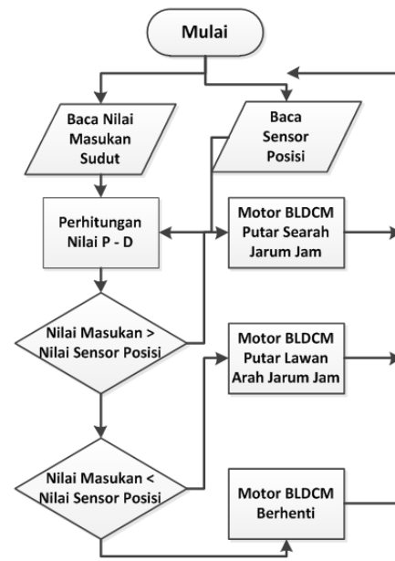
Gambar 4. Diagram flowchart
