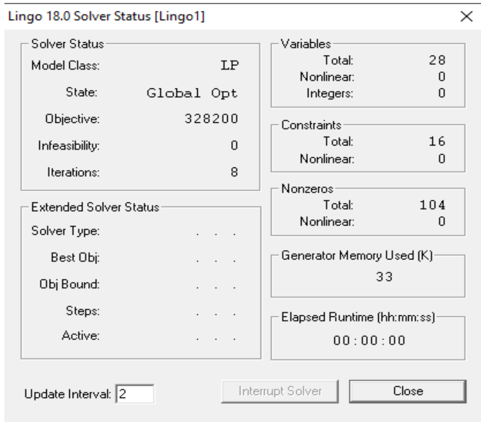
Figure 2. Output lingo application status
