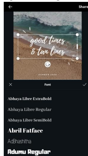
Figure 2. Template look
