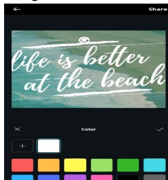
Figure 3. Canvas font
