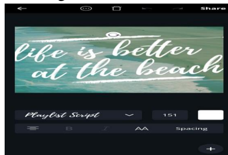
Figure 4. Canvas color
