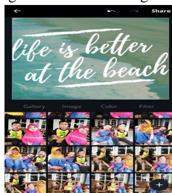
Figure 5. Canvas Background
