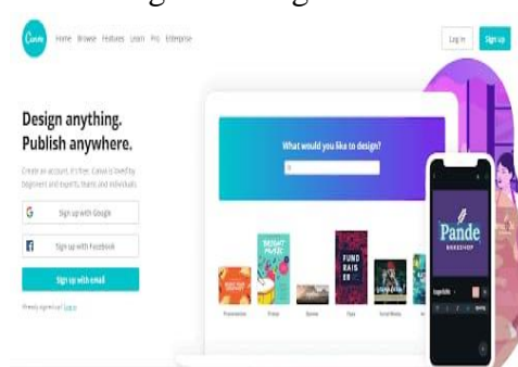
Figure 7. Login canva
