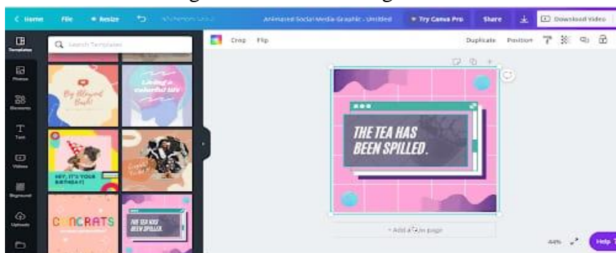
Figure 11. Custom design
