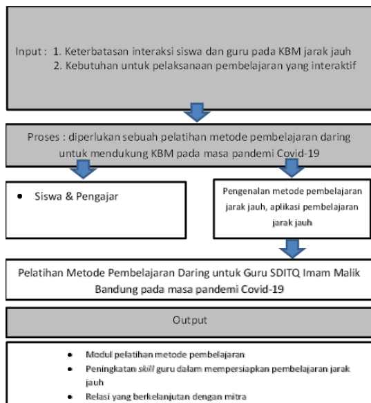
Gambar 1. Gambaran IPTEK
